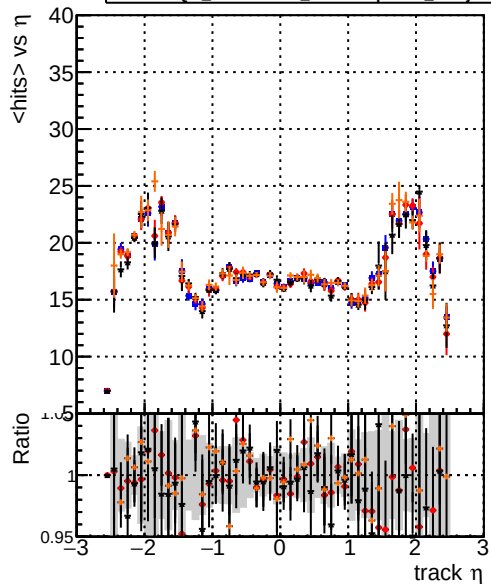
mean hit DQM_testMkFitFit_initialStepReso DQM_testMkFitFit_initialStepReso DQM_testMkFitFit_initialStepReso_wRejection10
