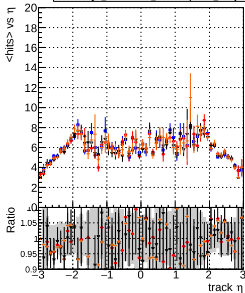
Legend: DQM_original4 (blue), DQM_testMkFit_initialStepReso (red), DQM_testMkFitFit_initialStepReso (black), DQM_testMkFitFit_initialStepReso_wRejection10 (orange) mean hit
