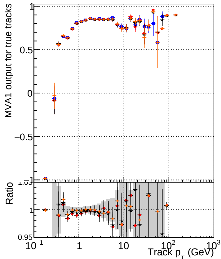
MVA1 of associated tracks (recoToSim) vs. track p_T
