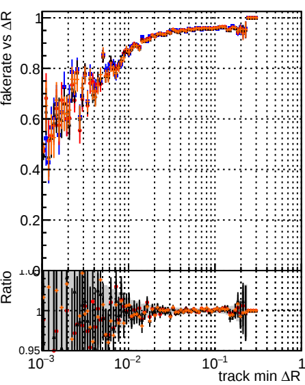
Fake rate vs \Delta R(\text{track, jet}) DQM original4 DQM testMKFit_initialStepReso DQM testMKFit_initialStepReso wRejection10
