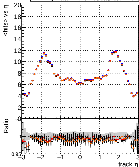
— DQM_original4 — DQM_testMkFit_initialStepReso — DQM_testMkFitFit_initialStepReso — DQM_testMkFitFit_initialStepReso_wRejection10 mean hits
