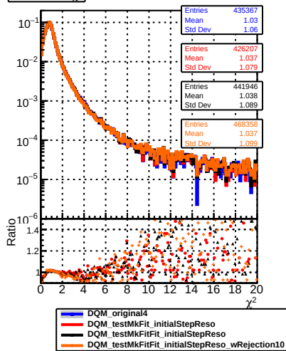
normalized \chi^2
