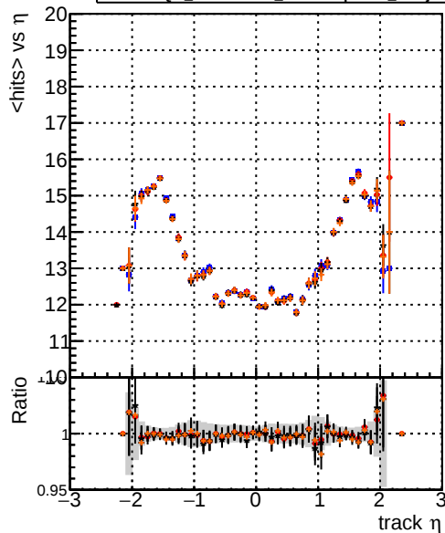
DQM_testMkFit_initialStepReso DQM_testMkFitFit_initialStepReso DQM_testMkFitFit_initialStepReso_wRejection10 DQM_testMkFitFit_initialStepReso mean hits
