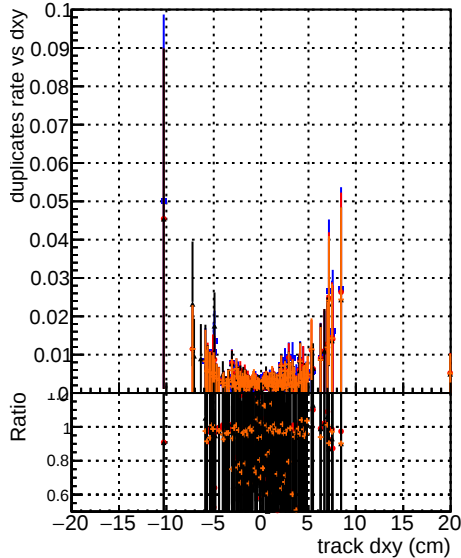
wRejection10
