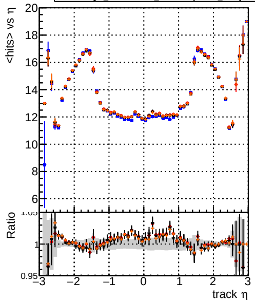
mean hit Legend: DQM_original4 (blue line), DQM_testMkFit_initialStepReso (red line), DQM_testMkFitFit_initialStepReso (black line), DQM_testMkFitFit_initialStepReso_wRejection10 (orange line)
