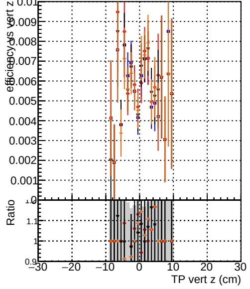
Efficiency vs. TP vert z — DQM_original4 — DQM_testMkFit_initialStepReso — DQM_testMkFitFit_initialStepReso — DQM_testMkFitFit_initialStepReso_wRejection10
