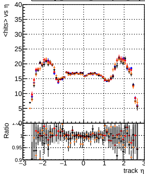
DQM_original4 DQM_testMkFit_initialStepReso DQM_testMkFitFit_initialStepReso DQM_testMkFitFit_initialStepReso_wRejection10 mean hit
