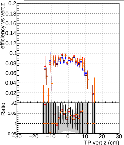
Efficiency vs vertpos DOM_original4 DOM_testMkFit_initialStepReso DOM_testMkFitFit_initialStepReso DOM_testMkFitFit_initialStepReso_Chi2Oneway
