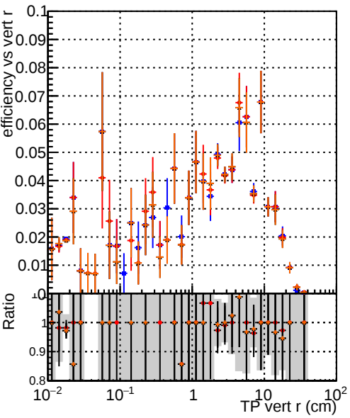
Efficiency vs vertpos Legend: DQM_original4 DQM_testMkFit_initialStepReso DQM_testMkFitFit_initialStepReso DQM_testMkFitFit_initialStepReso_chi2Oneway
