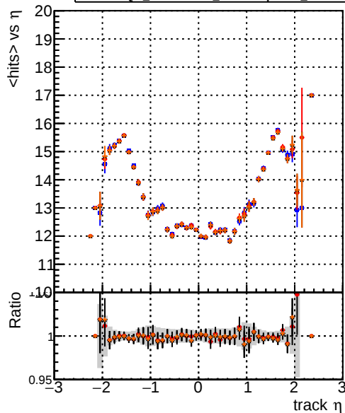
DQM_testMkFit_initialStepReso DQM_testMkFitFit_initialStepReso DQM_testMkFitFit_initialStepReso_Chi2Oneway mean hits
