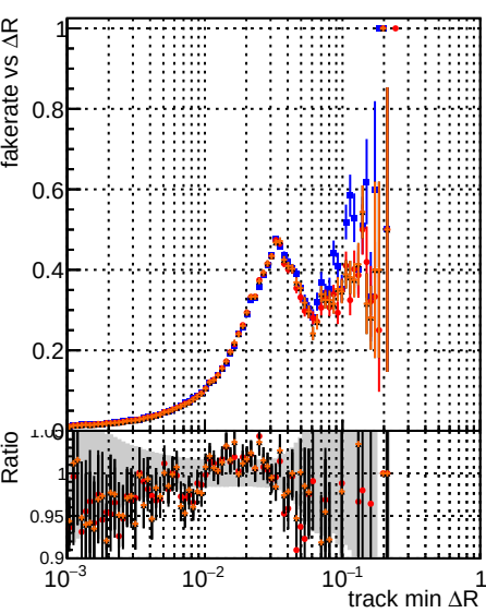
Fake rate vs \Delta R(\text{track, jet}) initialStepReso DOM test initialStepReso DOM fit initialStepReso DOM fit initialStepReso Chi2Oneway
