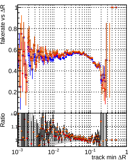
Fake rate vs \Delta R(\text{track, jet}) Duplicates Rate vs \Delta R(\text{track, jet}) Pileup rate vs \Delta R(\text{track, jet}) Ratio
