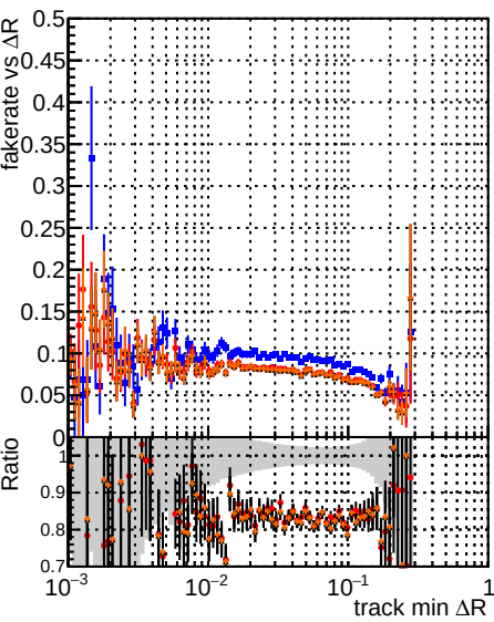
Fake rate vs \Delta R(\text{track, jet}) DOM original DOM test DOM fit DOM test fit initialStepReso testMKFit initialStepReso testMKFit initialStepReso Chi2Oneway
