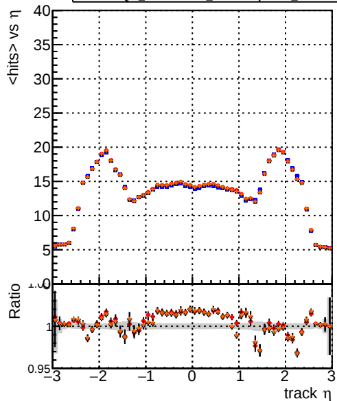
mean hits DQM_testMkFit_initialStepReso DQM_testMkFitFit_initialStepReso DQM_testMkFitFit_initialStepReso_Chi2Oneway
