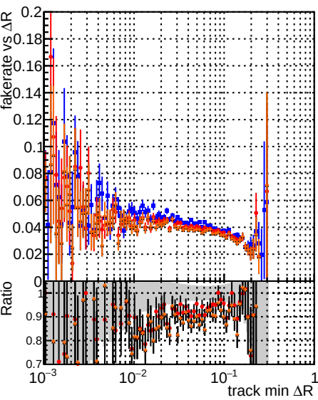
Fake rate vs \Delta R(\text{track, jet}) DOM original DOM test DOM test MKFit initialStepReso DOM test MKFit initialStepReso Chi2Oneway
