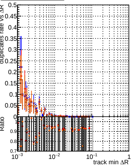
Fake rate vs \Delta R(\text{track, jet}) Duplicates Rate vs \Delta R(\text{track, jet}) Pileup rate vs \Delta R(\text{track, jet}) Chi2Oneway
