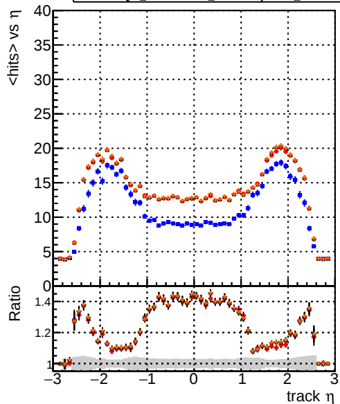
mean hit DQM_origina14 DQM_testMkFit_initialStepReso DQM_testMkFitFit_initialStepReso DQM_testMkFitFit_initialStepReso_Chi2Oneway
