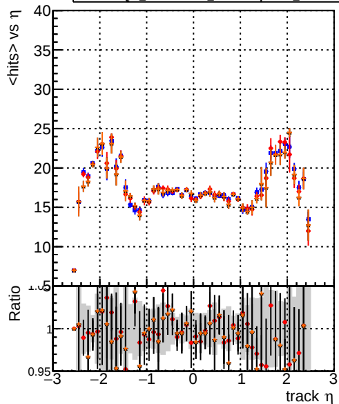
DQM_original4 DQM_testMkFit_fit_initialStepReso DQM_testMkFit_fit_initialStepReso DQM_testMkFit_fit_initialStepReso_chi2Oneway
