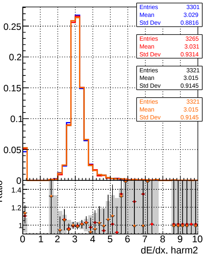
— DQM_original4 — DQM_testMkFit_initialStepReso — DQM_testMkFitFit_initialStepReso — DQM_testMkFitFit_initialStepReso_chi2Oneway
