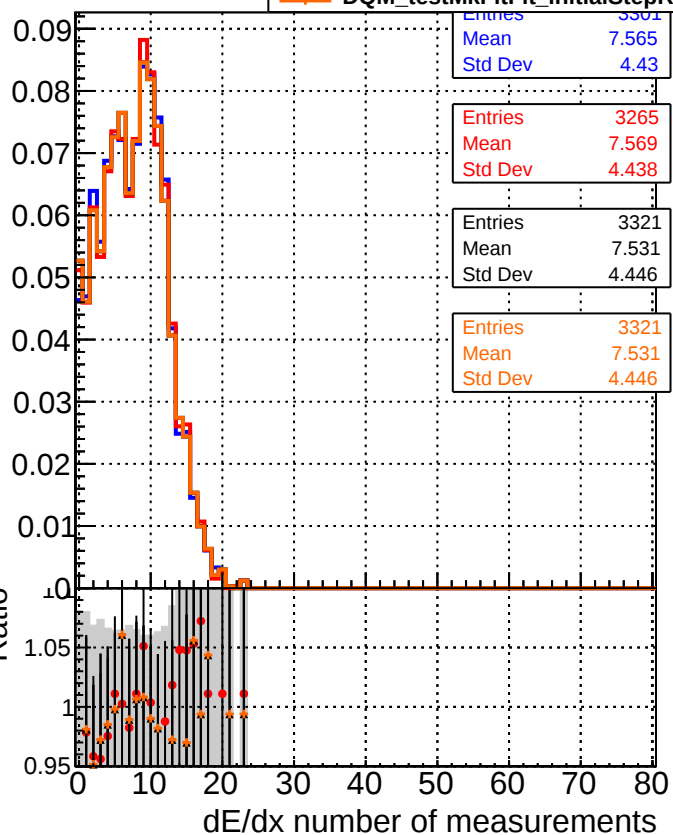
— DQM_original4 — DQM_testMkFit_initialStepReso — DQM_testMkFitFit_initialStepReso — DQM_testMkFitFit_initialStepReso_chi2Oneway
