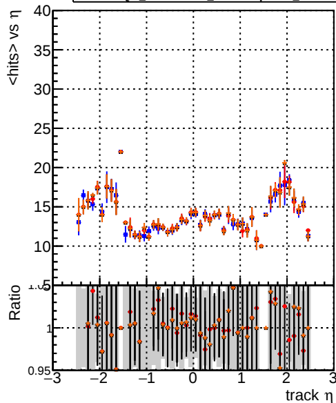
DQM_original4 DQM_testMkFit_initialStepReso DQM_testMkFitFit_initialStepReso DQM_testMkFitFit_initialStepReso_Chi2Oneway mean hits
