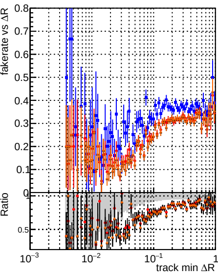
Fake rate vs \Delta R(\text{track, jet}) Legend: original4 testIMKFit testIMKFit_initialStepReso testIMKFit_initialStepReso_chi2oneway
