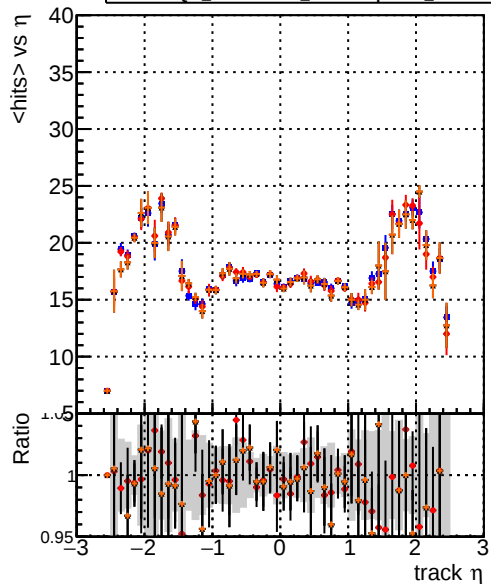
mean hits vs \eta DQM_original4 DQM_testMkFit_initialStepReso DQM_testMkFitFit_initialStepReso DQM_testMkFitFit_initialStepReso_Chi2Oneway
