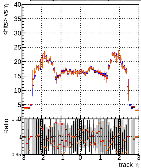
mean hit DQM_original4 DQM_testMkFit_fit_initialStepReso DQM_testMkFitFit_initialStepReso DQM_testMkFitFit_initialStepReso_Chi2Oneway
