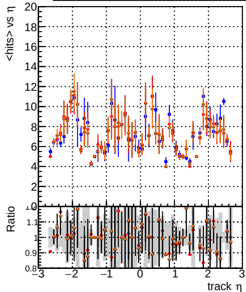
— DQM_testMkFitFit_initialStepReso — DQM_testMkFitFit_initialStepReso — DQM_testMkFitFit_initialStepReso — DQM_testMkFitFit_initialStepReso_chi2Oneway
