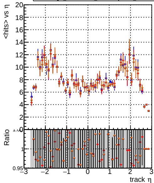
mean hit DQM_testMkFitFit_initialStepReso DQM_testMkFitFit_initialStepReso DQM_testMkFitFit_initialStepReso_Chi2Oneway
