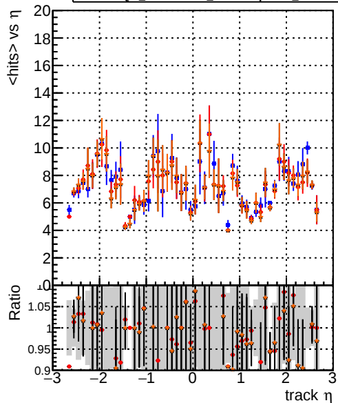
mean hits DQM_original4 DQM_testMkFit_fit_initialStepReso DQM_testMkFit_fit_initialStepReso DQM_testMkFit_fit_initialStepReso_chi2Oneway
