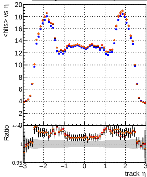
mean hit DQM_original4 DQM_testMkFit_initialStepReso DQM_testMkFitFit_initialStepReso DQM_testMkFitFit_initialStepReso_Chi2Oneway
