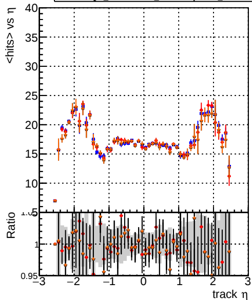
mean hits DQM_original4 DQM_testMkFit_initialStepReso DQM_testMkFitFit_initialStepReso DQM_testMkFitFit_initialStepReso_chi2Oneway
