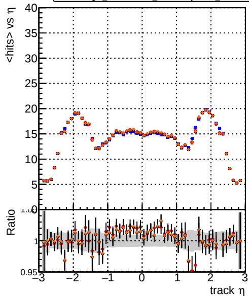
mean hit DQM_original4 DQM_testMkFit_initialStepReso DQM_testMkFitFit_initialStepReso DQM_testMkFitFit_initialStepReso_Chi2Oneway
