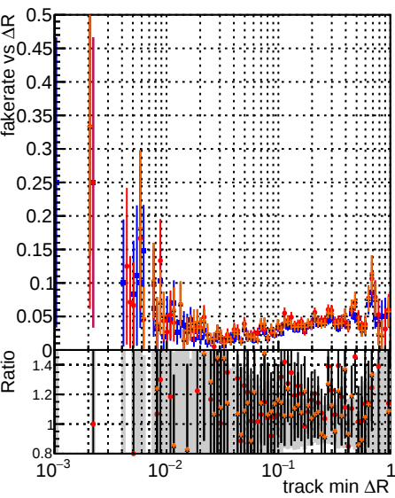
Fake rate vs \Delta R(\text{track, jet}) DQM original4 DQM testMKFit_initialStepReso DQM testMKFit_initialStepReso_chi2oneway
