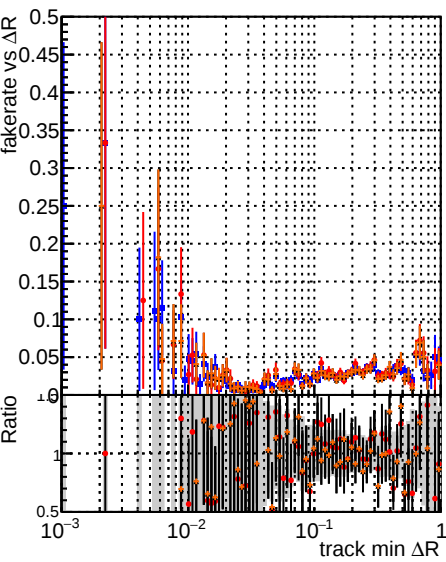
Fake rate vs \Delta R(\text{track, jet}) Legend: DOM original (blue squares) DOM test (red circles) DOM fit (black triangles) DOM fit initialStepReso (orange diamonds) Chi2Oneway
