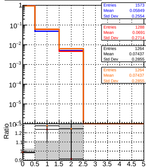
mean hit — DQM_original4 — DQM_testMkFit_initialStepReso — DQM_testMkFitFit_initialStepReso — DQM_testMkFitFit_initialStepReso_chi2Oneway
