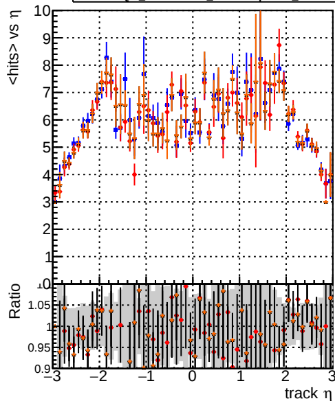
mean hits DQM_original4 DQM_testMkFit_initialStepReso DQM_testMkFitFit_initialStepReso DQM_testMkFitFit_initialStepReso_Chi2Oneway
