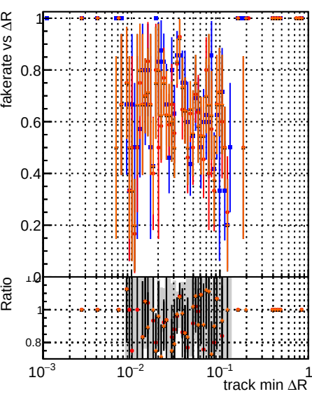
Fake rate vs \Delta R(\text{track, jet}) DQM original4 DQM testIMKFit_initialStepReso DQM testIMKFit_initialStepReso_chi2oneway
