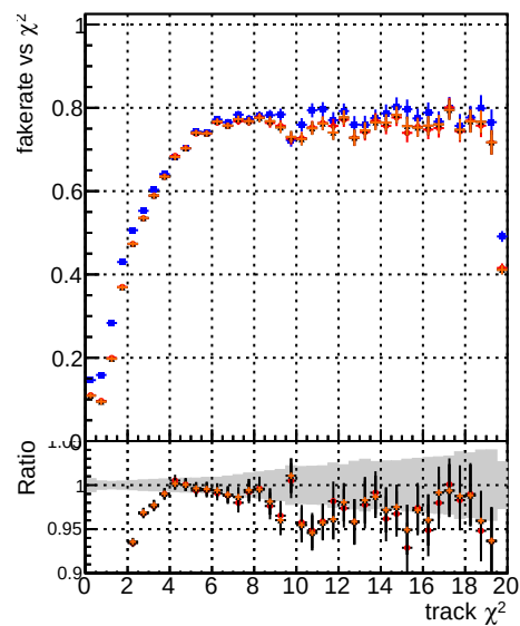
Fake rate vs. \chi^2 Legend: DOM original, DOM test, MRFF, FF, InitialStepReso, Chi2Oneway
