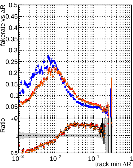
Fake rate vs \Delta R(\text{track, jet}) Chi2Oneway
