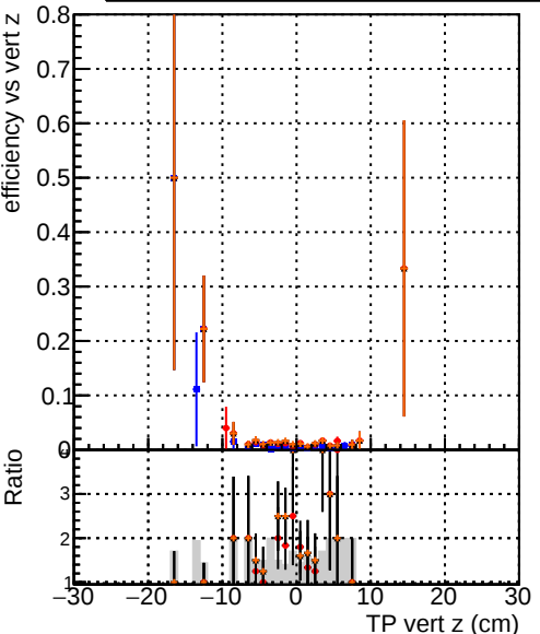
Efficiency vs vertpos DQM_original4 DQM_testMkFit_initialStepReso DQM_testMkFitFit_initialStepReso DQM_testMkFitFit_initialStepReso_Chi2Oneway
