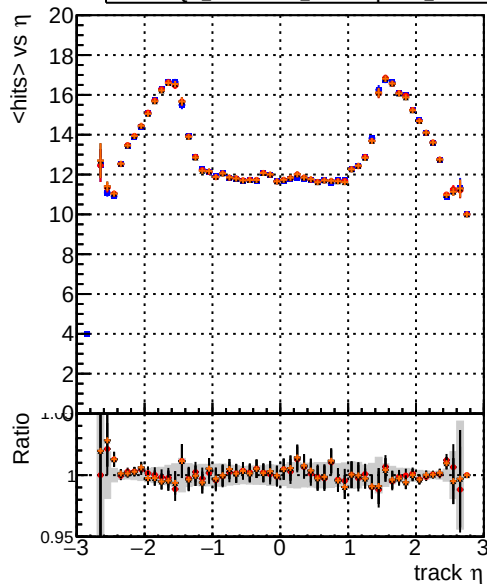
mean hits DQM_origina14 DQM_testMkFit_initialStepReso DQM_testMkFitFit_initialStepReso DQM_testMkFitFit_initialStepReso_Chi2Oneway
