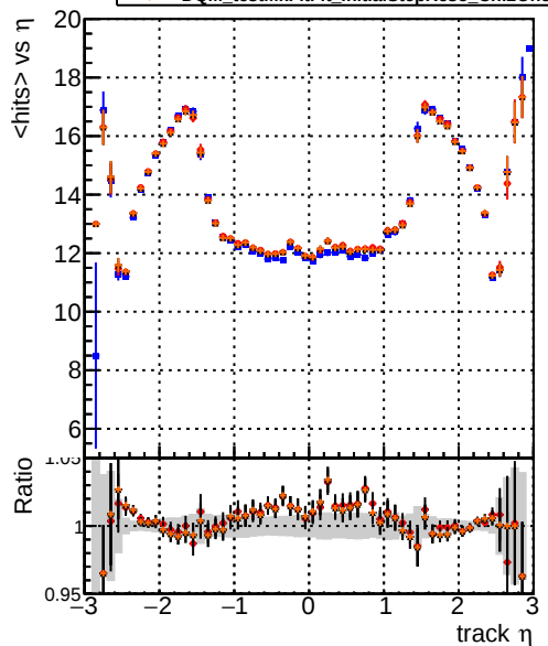
mean hits vs \eta Legend: DQM_original4 (blue line), DQM_testMkFit_fit_initialStepReso (red line), DQM_testMkFit_fit_initialStepReso (black line), DQM_testMkFit_fit_initialStepReso_chi2Oneway (orange line)
