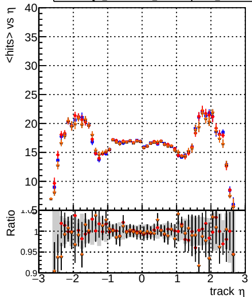
DQM_original4 DQM_testMkFit_initialStepReso DQM_testMkFitFit_initialStepReso DQM_testMkFitFit_initialStepReso_Chi2Oneway mean hits
