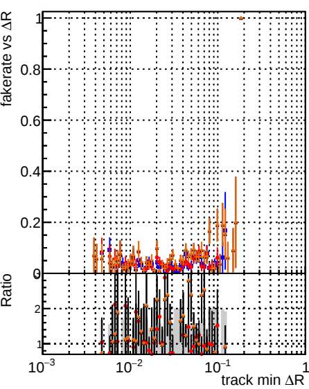
Fake rate vs \Delta R(\text{track, jet}) DQM original4 DQM testIMKFit initialStepReso DQM testIMKFit initialStepReso DQM testIMKFit initialStepReso Chi2Oneway
