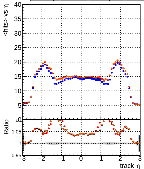
mean hits DQM_original4 DQM_testMkFit_initialStepReso DQM_testMkFitFit_initialStepReso DQM_testMkFitFit_initialStepReso_Chi2Oneway
