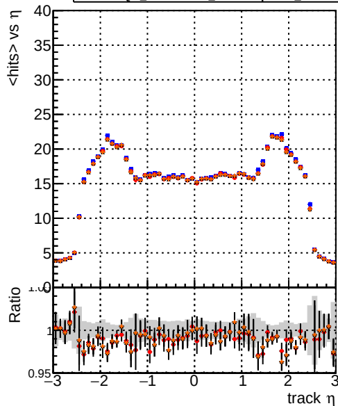
mean hits DQM_original14 DQM_testMkFit_initialStepReso DQM_testMkFitFit_initialStepReso DQM_testMkFitFit_initialStepReso_Chi2Oneway
