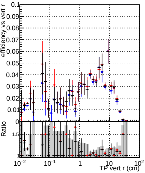
Efficiency vs TP vert r (cm) DQM_original DQM_firstTest_byPassRefit DQM_firstTestFit4_1000ev
