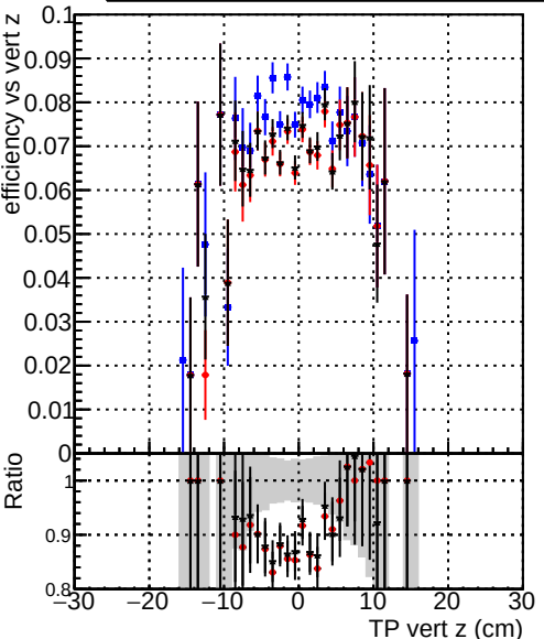
Efficiency vs TP vert z (cm) Legend: DQM_original (blue stars) DQM_firstTest_byPassRefit (red stars) DQM_firstTestFit4_1000ev (black stars)
