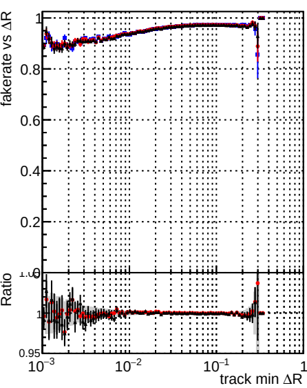
Fake rate vs \Delta R (track, jet) Legend: - DQM_original (blue line with dots) - DQM_firstTest_byPassRefit (red line with dots) - DQM_firstTestFit4_1000ev (black line with dots)
